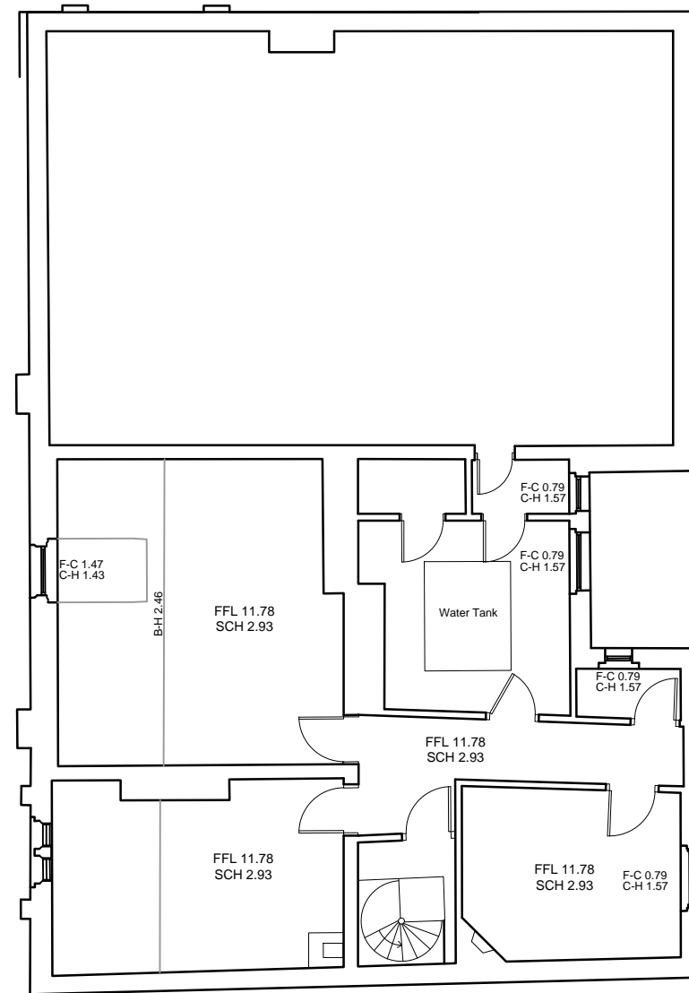
SECOND FLOOR @ 1:125
