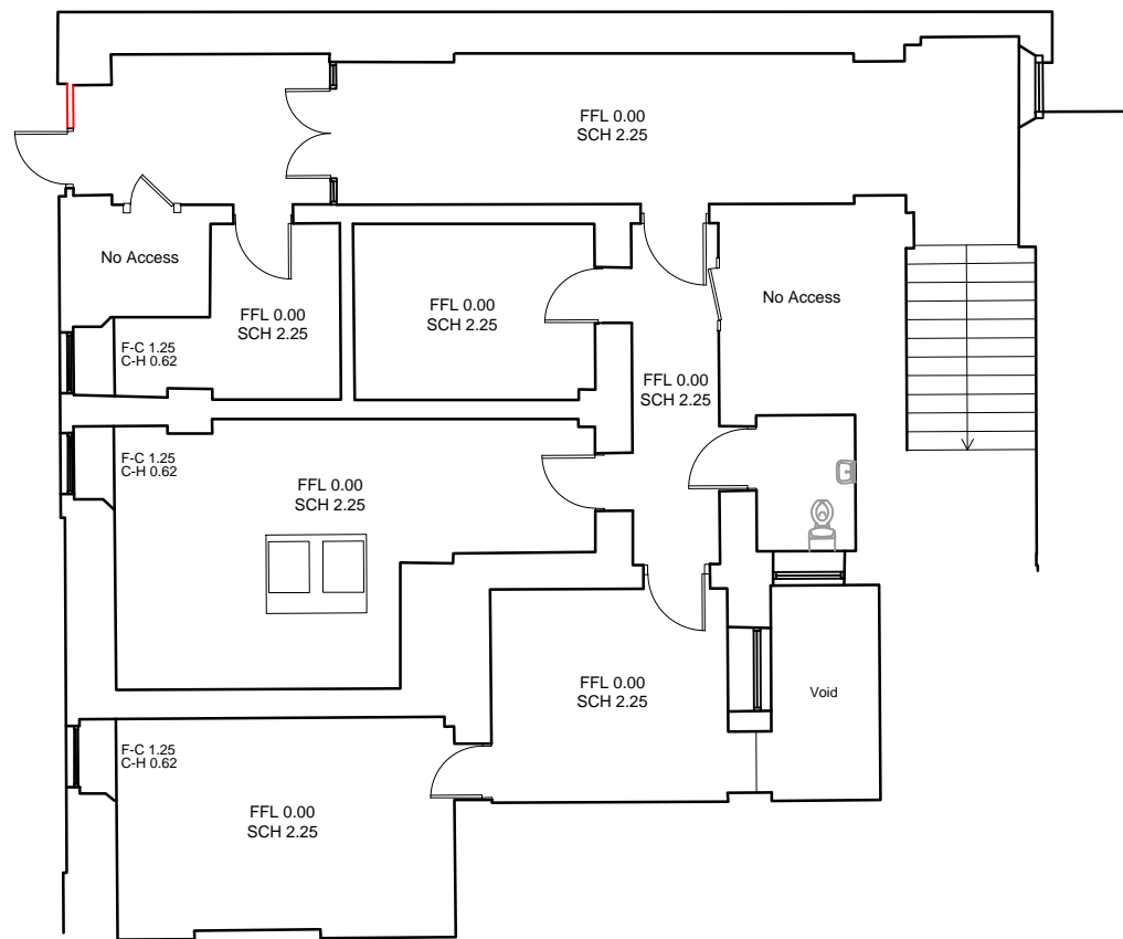
LOWER GROUND FLOOR @ 1:125
