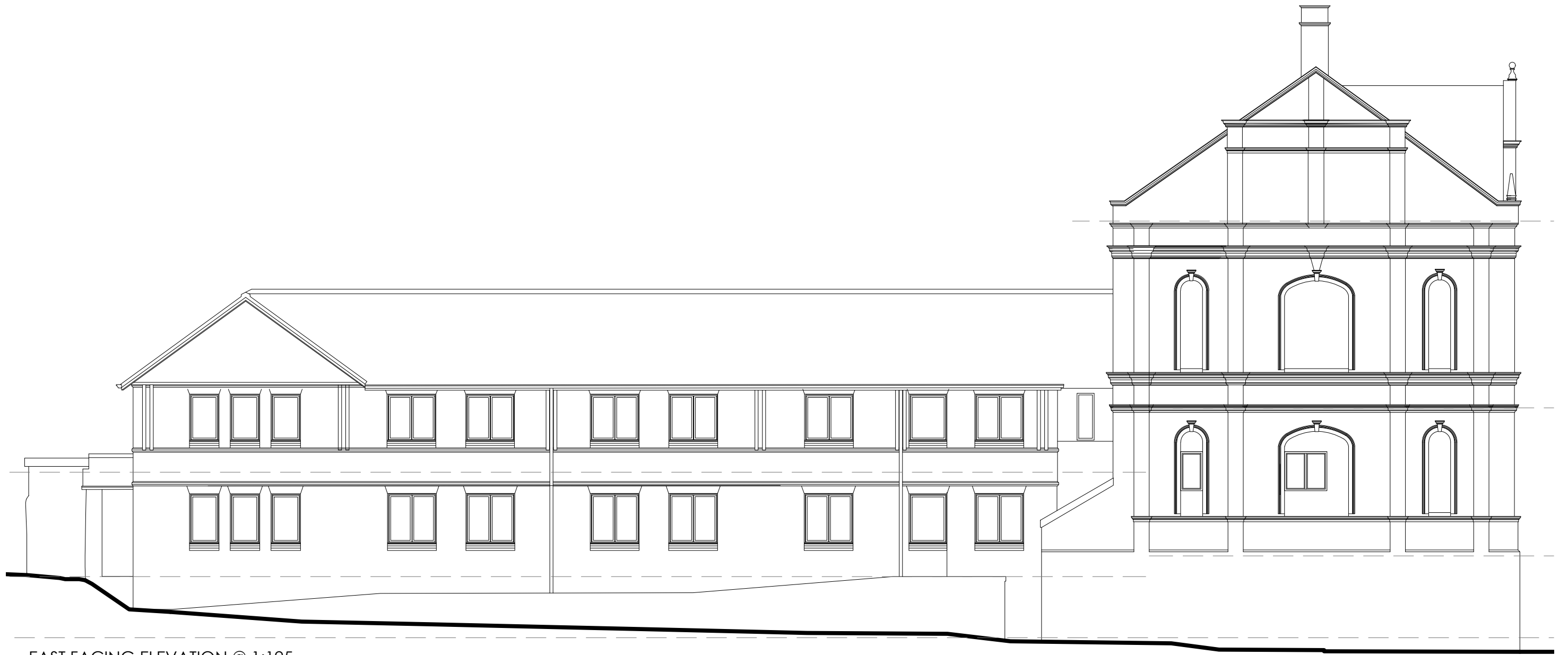
EAST FACING ELEVATION @ 1:125
