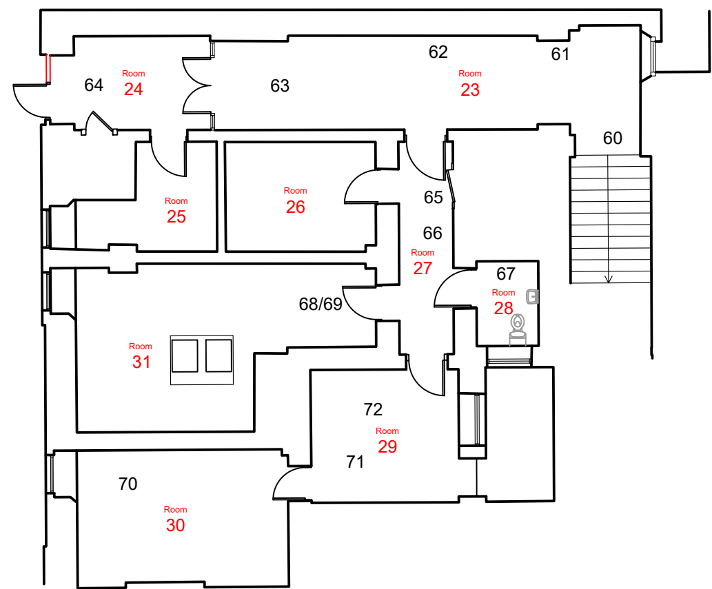
BASEMENT @ 1:125
