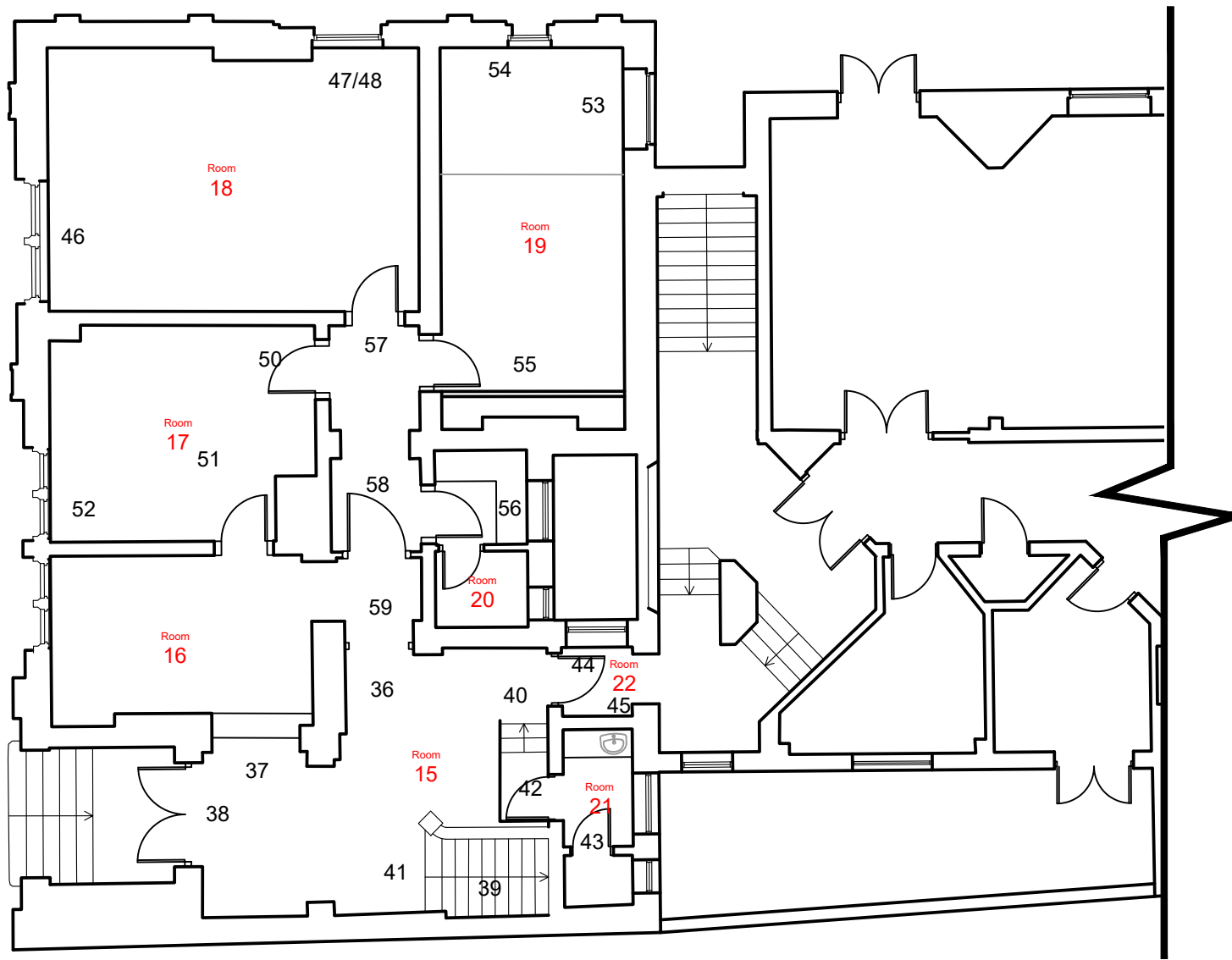
GROUND FLOOR (PARTIAL) @ 1:125
