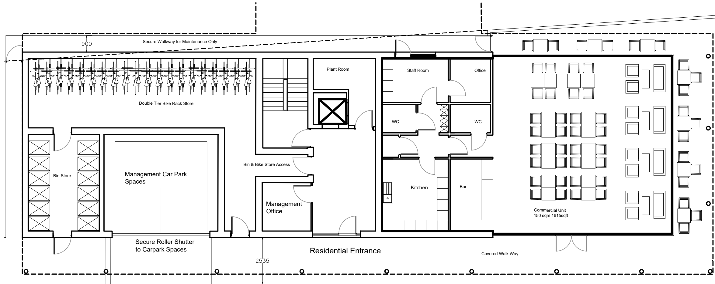
Ground Floor Plan 1:125 @ A3
