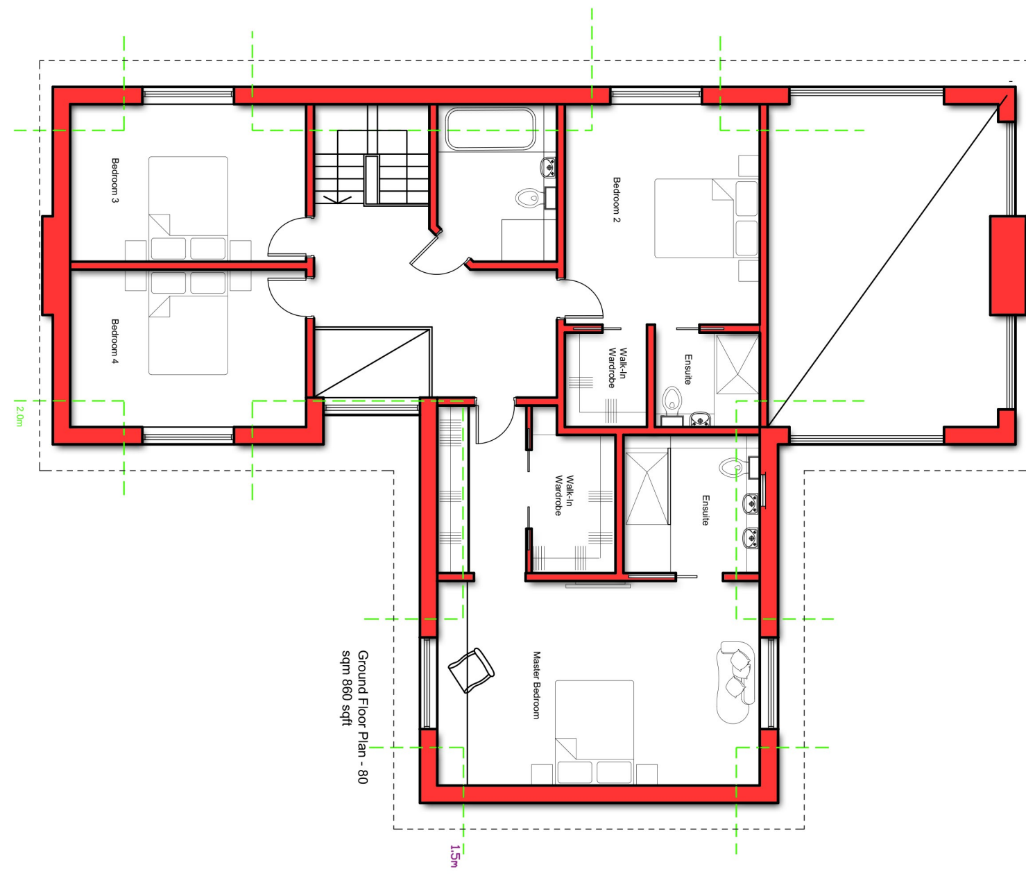
First Floor Plan 1:100 @ A3
