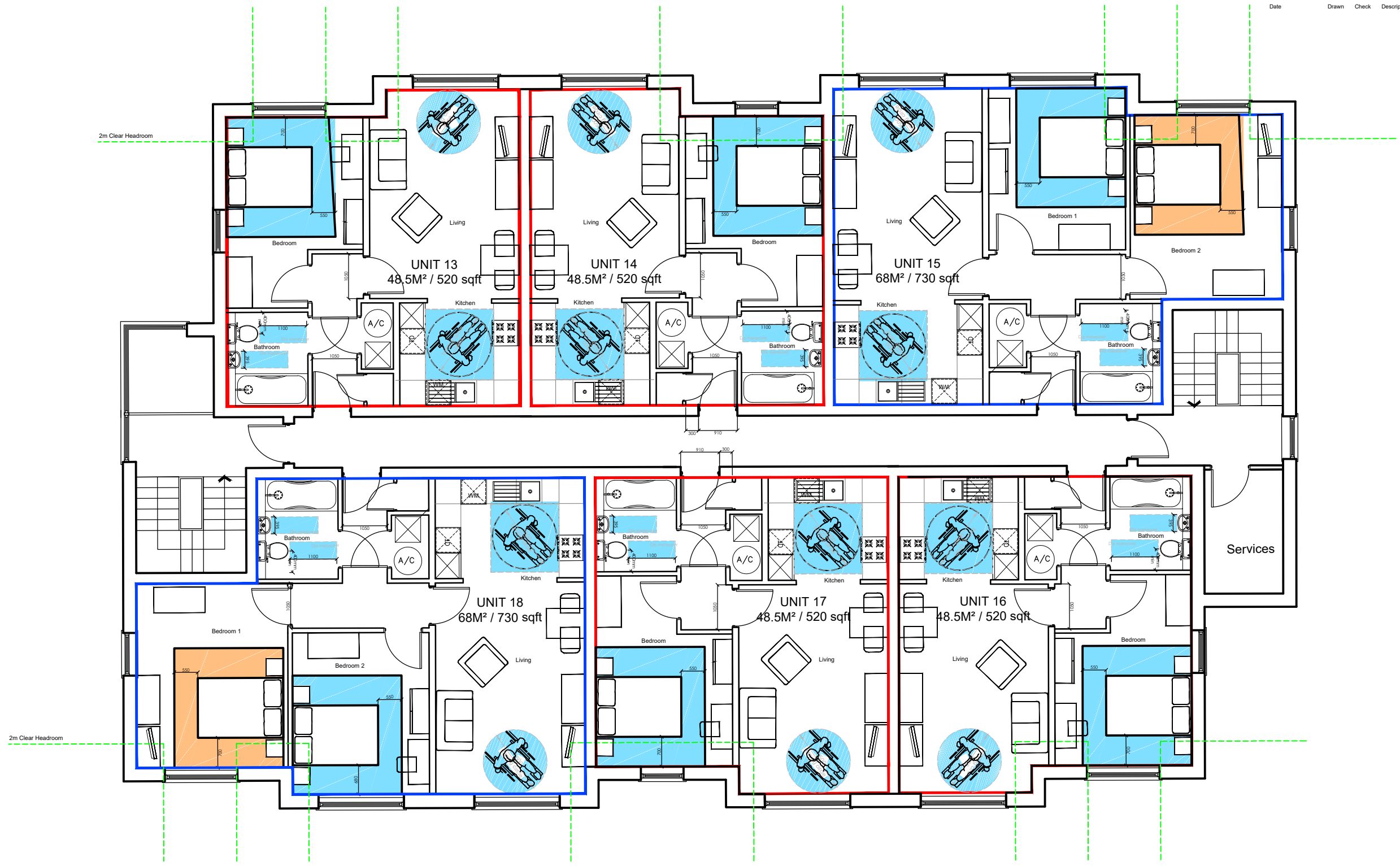
Proposed 2nd Floor Plan
