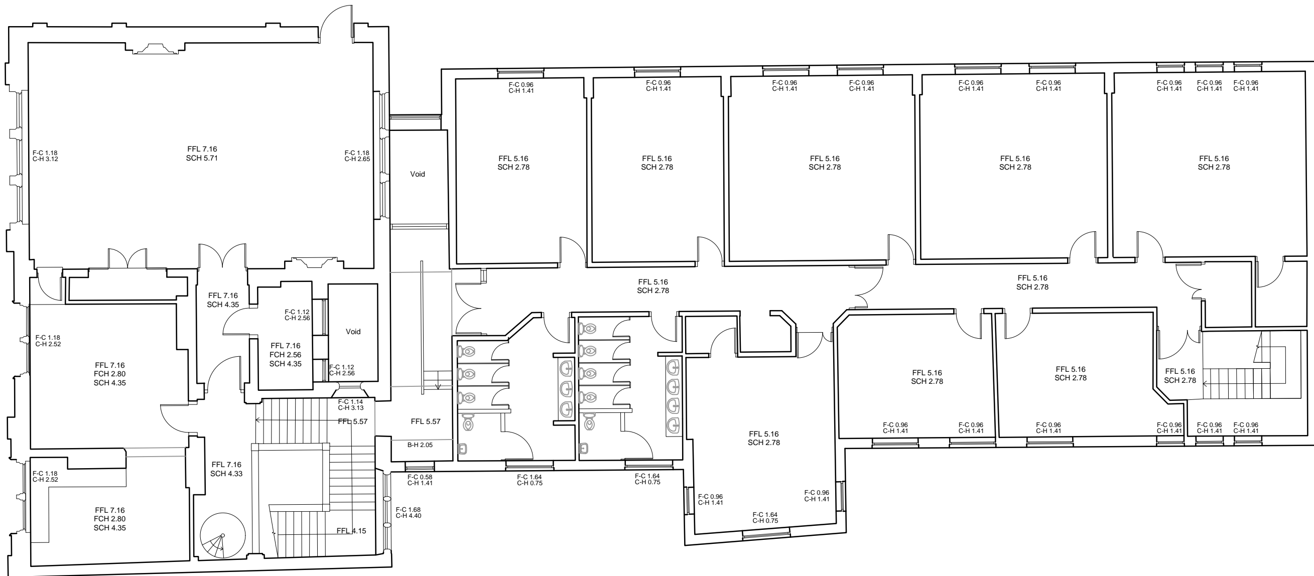
FIRST FLOOR @ 1:125
